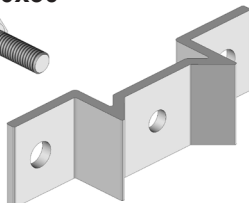
DIN933M10x30
